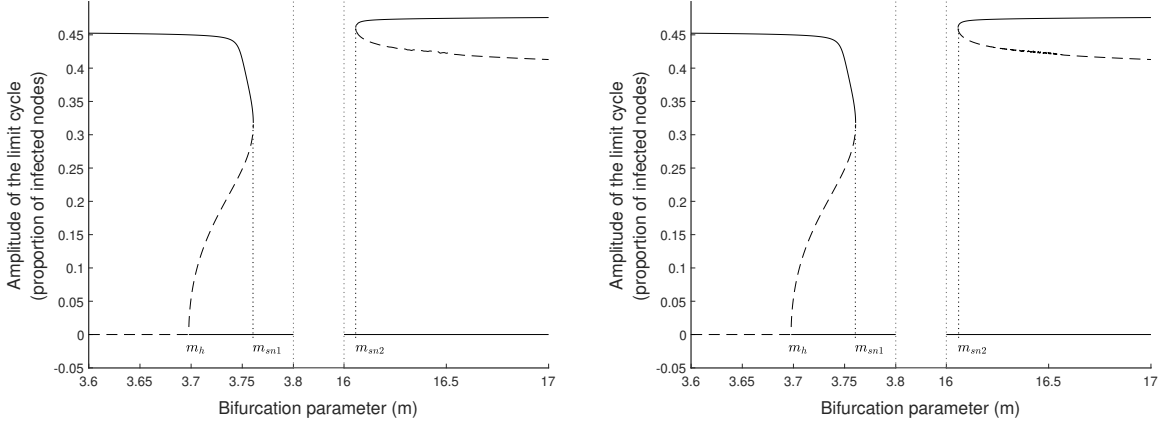
Figure 5: Bifurcation diagram for \varepsilon = 0 (left) and \varepsilon = 10^{-5} (right).
