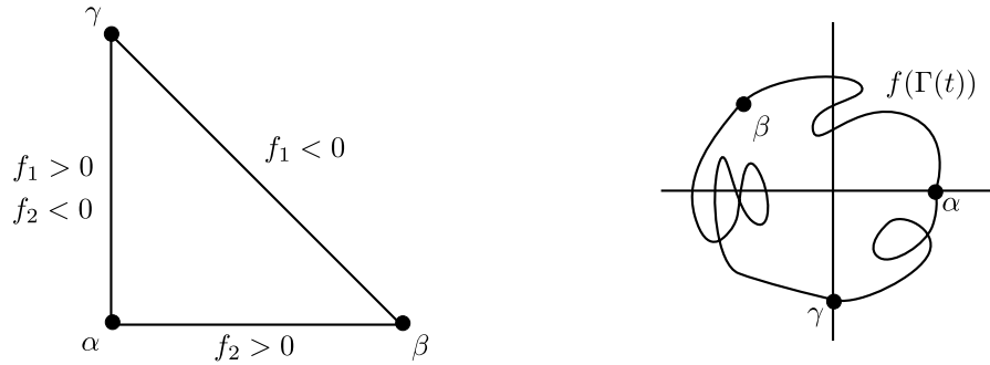
Figure 11: On the left, structure and assumptions of the Poincaré-Miranda theorem for triangles in Theorem 6.2. On the right, an sketch of the behaviour of the function f(\Gamma(t)) for t \in [0, 1] .
