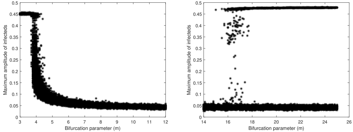
Figure 9: Maximum amplitude of each GA output in the time interval [1000, 10000] . Parameters of the simulation: N = 10^5 .
