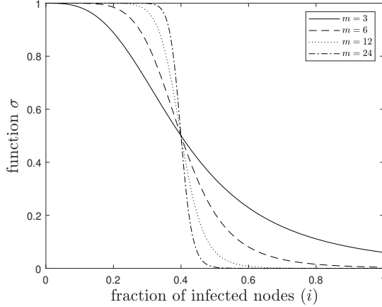
Figure 1: Shape of function \sigma_m(i) with \eta = 0.4 for different values of m .
