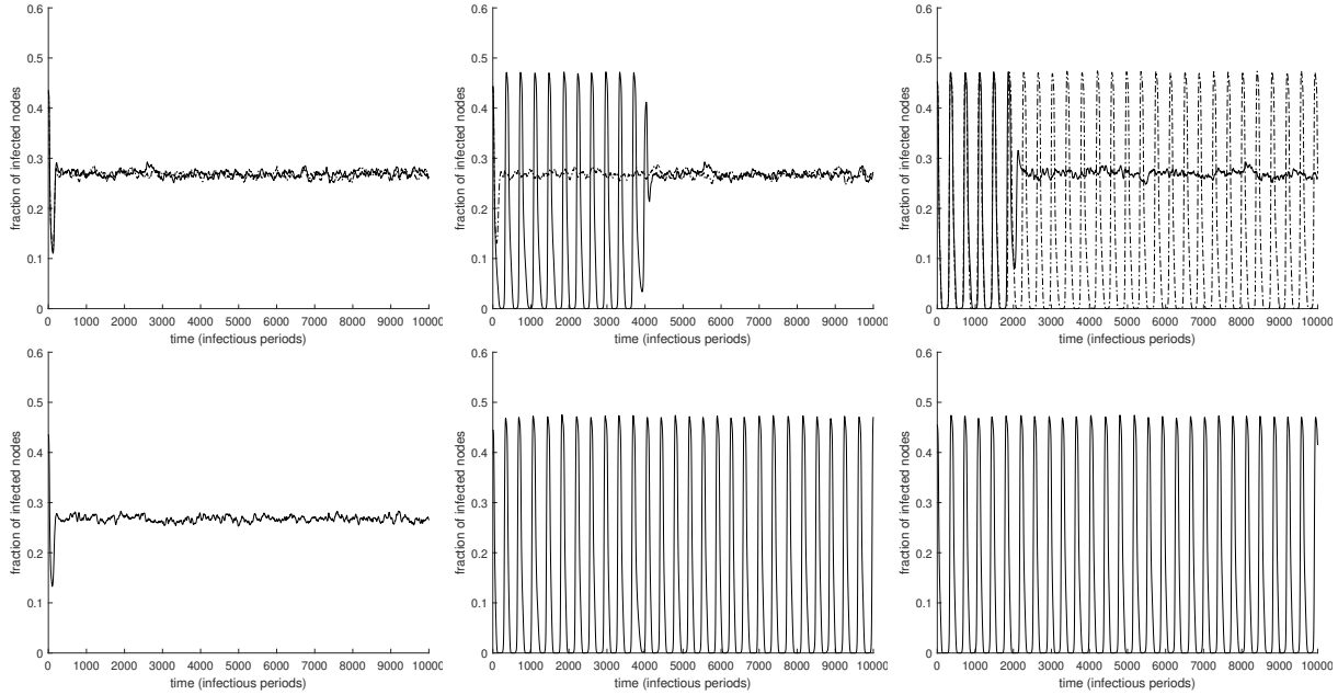
Figure 8: On top, two outputs from GA with parameter m = 17 and initial conditions a_0 = 0.033240 , i_0 = 0.437330 , u_0 = 0.039240 (left), a_0 = 0.033240 , i_0 = 0.447330 , u_0 = 0.025900 (center), a_0 = 0.033240 , i_0 = 0.457330 , u_0 = 0.012570 (right). On bottom, a single output from GA with parameter m = 18 and initial conditions a_0 = 0.033240 , i_0 = 0.437420 , u_0 = 0.039140 (left), a_0 = 0.033240 , i_0 = 0.447420 , u_0 = 0.025810 (center), a_0 = 0.033240 , i_0 = 0.457420 , u_0 = 0.012480 (right). Parameters of the simulation: N = 10^5 .
