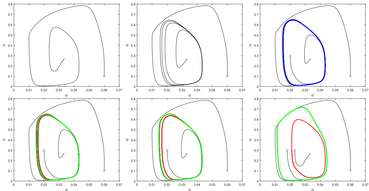
Figure 4: Projections on the (a, u) -plane of some solutions of system (1) for m = 16 (top left), m = 16.05 (top middle), m = 16.0575 (top right), m = 16.05755 (bottom left), m = 16.06 (bottom middle) and m = 17 (bottom right). The orbit in green corresponds to the hyperbolic attractive limit cycle, the orbit in red to the hyperbolic repulsive limit cycle and the orbit in blue to the non-hyperbolic semistable limit cycle. Blue circles mark the initial conditions.
