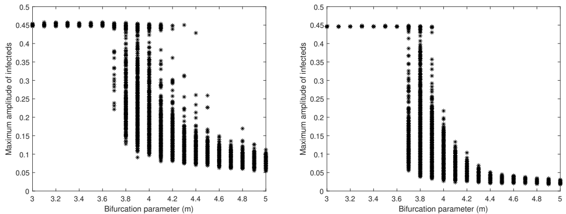
Figure 10: Maximum amplitude of each GA output in the time interval [1000, 10000] . Parameters of the simulation: N = 10^5 (left). N = 10^6 (right).
