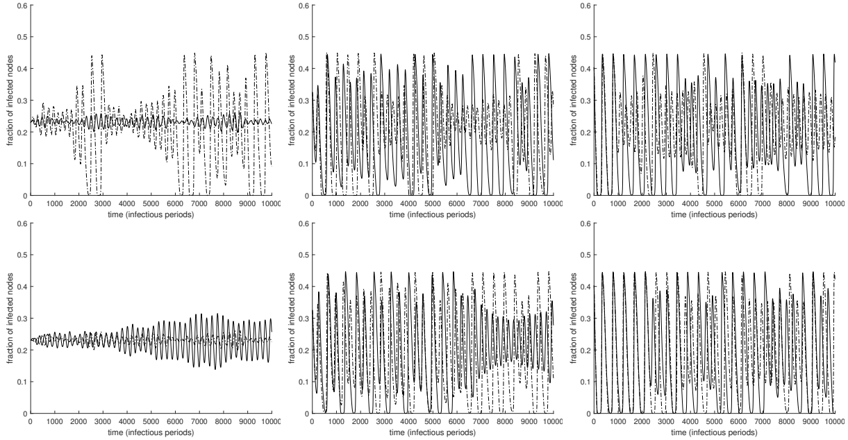
Figure 7: On top, two outputs from GA with parameter m = 3.7 with N = 10^5 (dotted line) and N = 10^6 (solid line), and initial conditions a_0 = 0.039359 , i_0 = 0.231104 , u_0 = 0.306049 (left), a_0 = 0.039359 , i_0 = 0.331104 , u_0 = 0.172716 (center), a_0 = 0.039359 , i_0 = 0.431104 , u_0 = 0.039382 (right) and same initial random seed. On bottom, two outputs from GA with parameter m = 3.7 with N = 10^6 and same initial conditions as before with different initial random seed.
