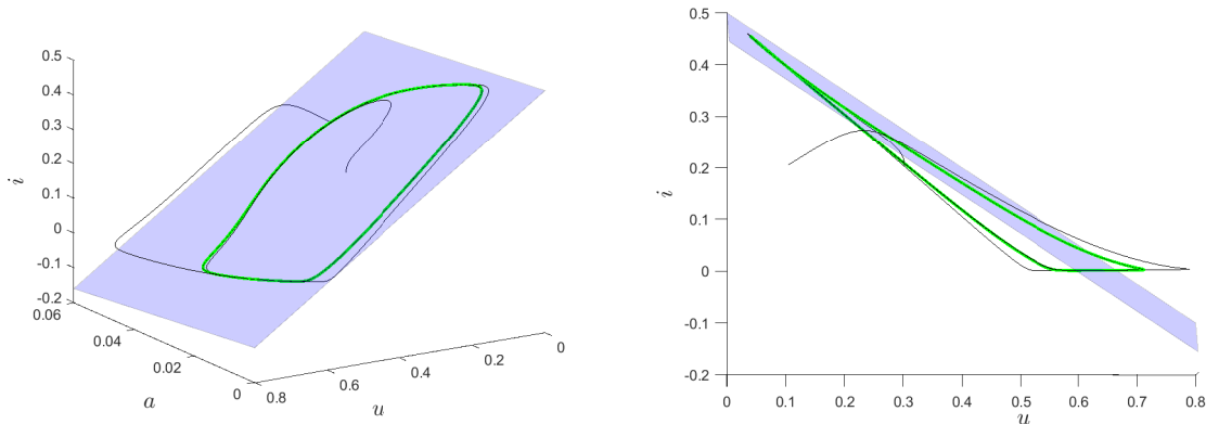
Figure 2: Two solutions of system (1) for m = 3.5 tending to the limit cycle (in green) whose dynamics is close to the plane (2) (in light blue).
