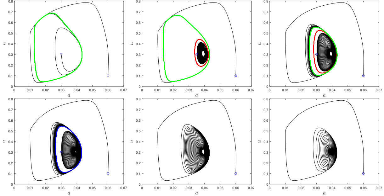
Figure 3: Projections on the (a, u) -plane of some solutions of system (1) for m = 3.69 (top left), m = 3.73 (top middle), m = 3.76 (top right), m = 3.76082 (bottom left), m = 3.77 (bottom middle) and m = 3.8 (bottom right). The orbit in green corresponds to the hyperbolic attractive limit cycle, the orbit in red to the hyperbolic repulsive limit cycle and the orbit in blue to the non-hyperbolic semistable limit cycle. Blue circles mark the initial conditions.
