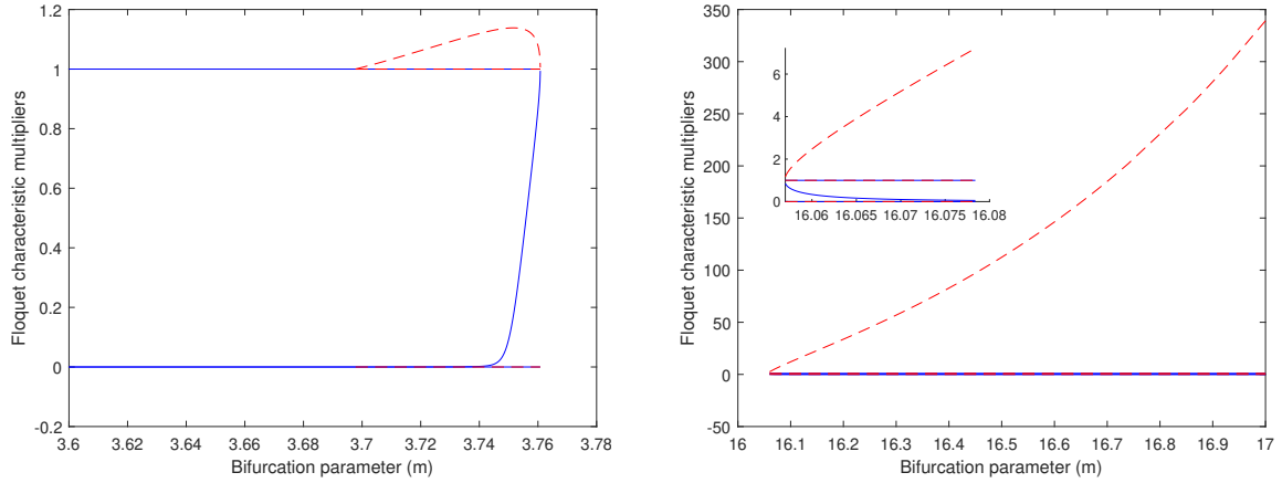
Figure 6: Floquet characteristic multipliers of the stable limit cycle (solid blue line) and the unstable limit cycle (dashed red line).
