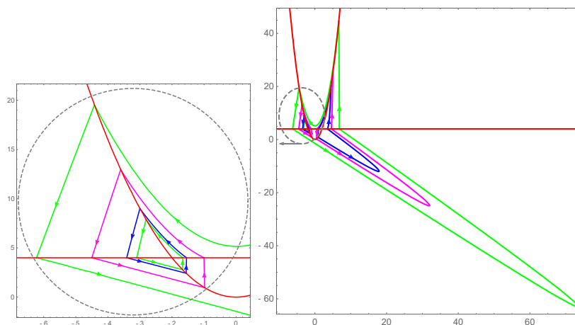
FIGURE 19. Two limit cycles with Conf 6 + , three limit cycles with Conf 6 - and one limit cycle with Conf 8 of system (38).
