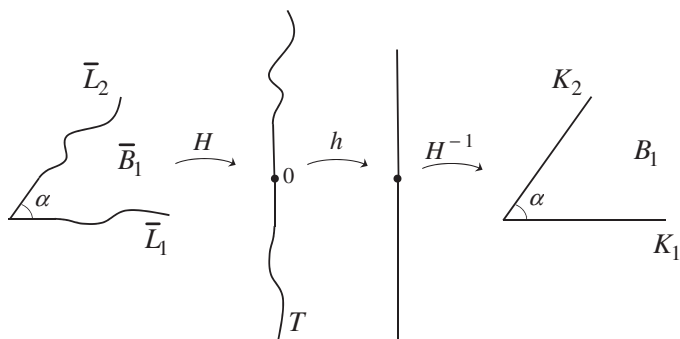
Fig. 3. Construction of \psi_1 := H^{-1} \circ h \circ H to regularise one sector of the topological star \bar{L} .
