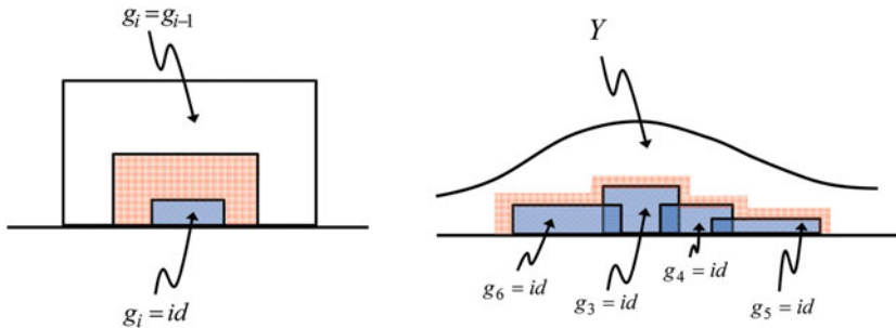
Fig. 5. (Colour online) Construction of g_i and overlapping of the successive modifications.
