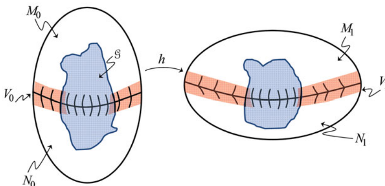
Fig. 1. (Colour online) An illustration of the assumptions of Theorem 3.2 (b).
