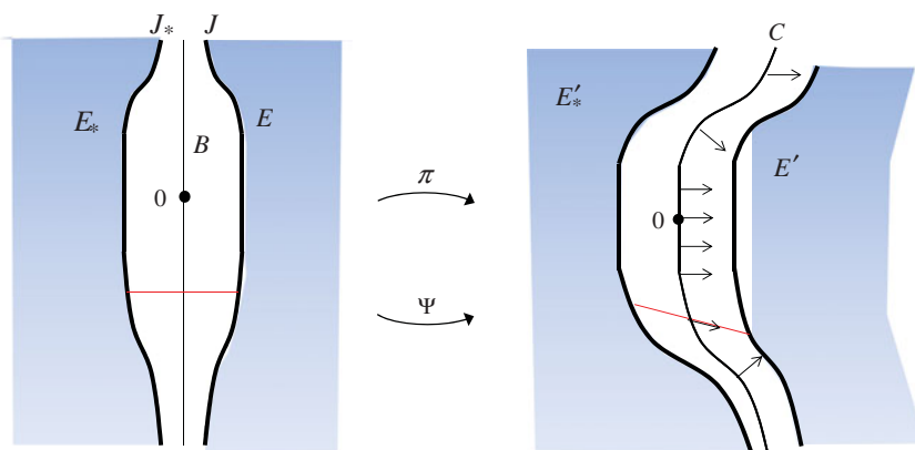
Fig. 2. (Colour online) C^k -diffeomorphisms, \pi : B \rightarrow \pi(B) , \psi : E \rightarrow E' .
